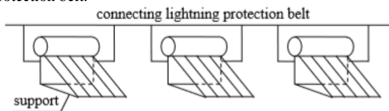
Fig.5. Lightning belt protection for several solar water heaters
