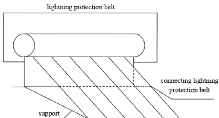
Fig.4. Lightning belt protection for solar water heaters
