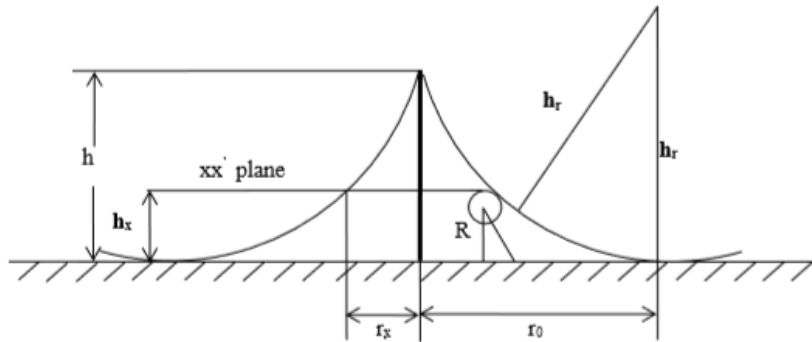
Fig.3. A single lightning rod protection for solar water heaters
