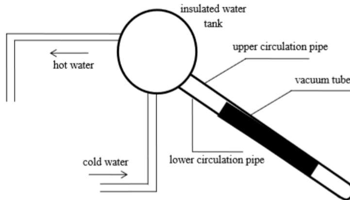
Fig.1. Principle of solar water heaters
